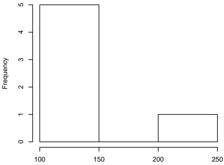
Gly
