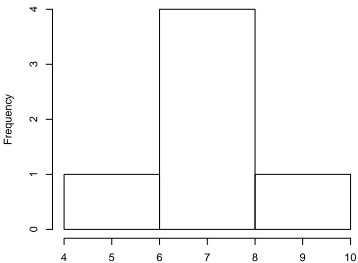
Lys
