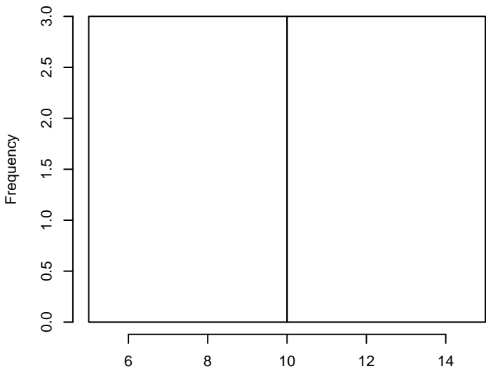
Tyr
