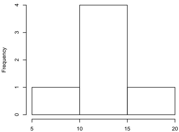
Val
