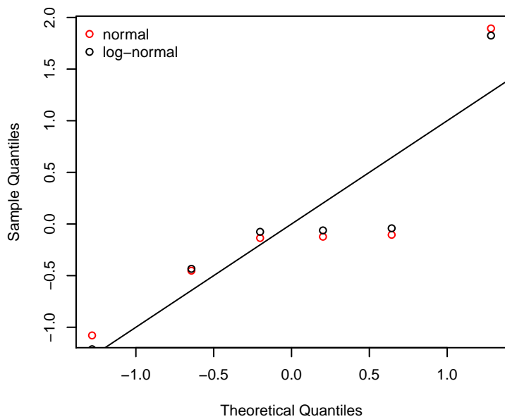
Q-Q Plot
