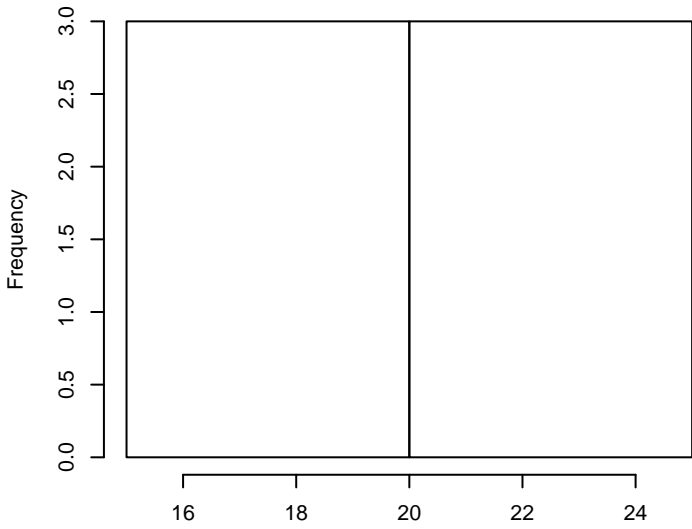
Arg
