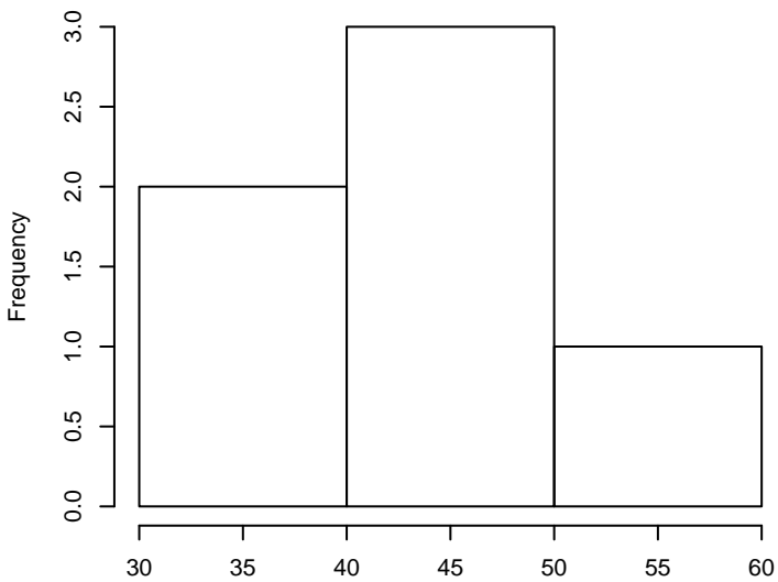
Asn
