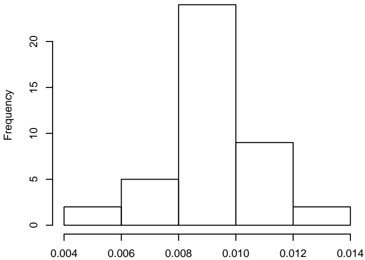
Asn
