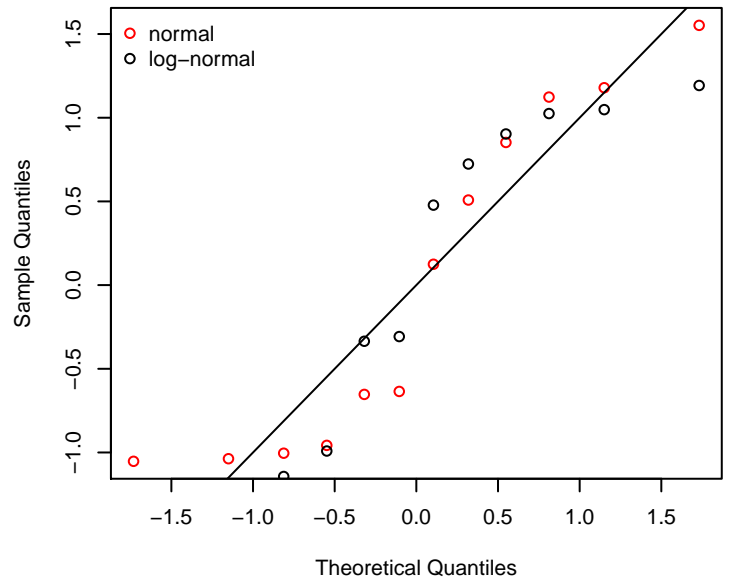
Q-Q Plot
