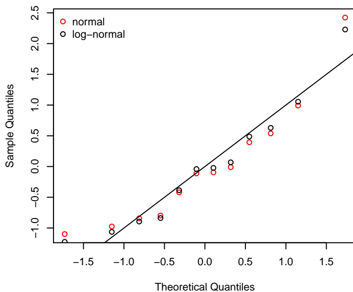
Q-Q Plot
